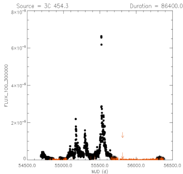
Fig. 3. Average daily flux ( E > 100 MeV) seen by the Fermi LAT for blazar 3C 454.3 from the start of the Fermi science mission (2008 August) until 2013 March. Red arrows (primarily clustered along the x-axis with the arrowheads invisible) indicate days in which the blazar was not detected † .
