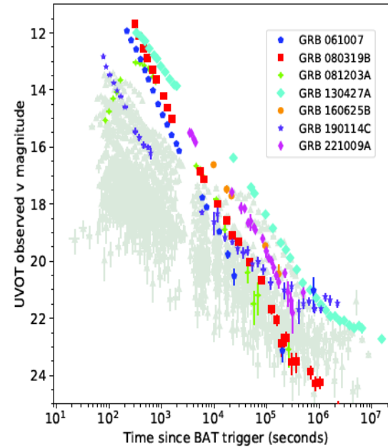
Figure 4. A sample of long GRB UVOT light curves. Those in colour are the brightest observed by UVOT (see Section 4.1) and include GRB 061007, GRB 080319B, GRB 081203A, GRB 160625B, GRB 190114C, and GRB 221009A. The grey light curves are UVOT-observed GRBs discovered between 2005 and 2010, taken from [61]. To create each light curve, individual colour filters ( b , u , uvw1 , uvm2 , uvw2 , and white ) were normalised to the v -band light curve and were co-added to construct a single filter, v -band, and light curve. These light curves have not been corrected for extinction. For the light curves highlighted in colour, the extinction is small A_v < 0.5 mag, except for GRB 221009A, which has a significant extinction with A_v = 4.1 mag [169].
