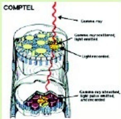
Compton telescopes
