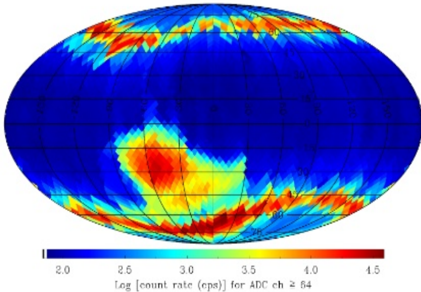
Fig. 9. The particle background, the extra-galactic X-ray and secondary (albedo) X-ray background radiation as measured by the detector system of GRBAlpha . Data plotted here are acquired during the commissioning phase and contains nearly 2 days of continuous measurements along the orbit of GRBAlpha . The northern and southern polar regions as well as the South Atlantic Anomaly are clearly visible with the elevated background levels. Otherwise, the background level is around 100 counts/sec in the full spectral range. On this map, an equal-area Mollweide geographical projection is used where the prime meridian and the equator crosses the center.
