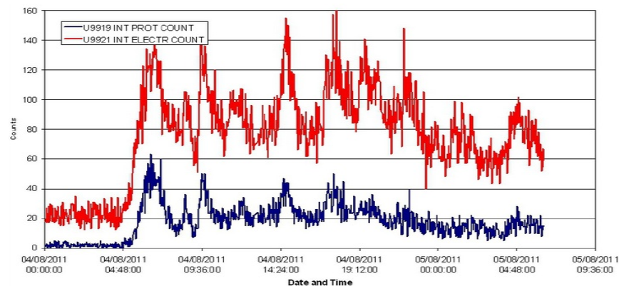
Figure 35: IREM (INTEGRAL Radiation Environment Monitor) output in Solar Flare (image credit: ESA)
