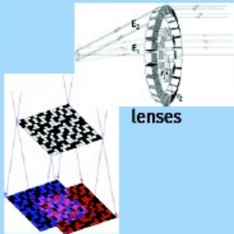
coded masks
