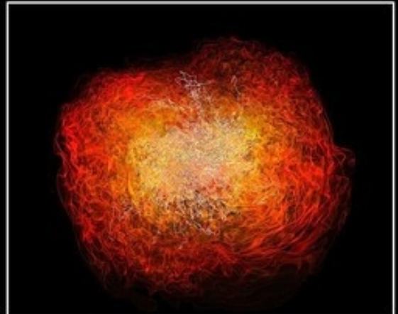
13.8 milliseconds
