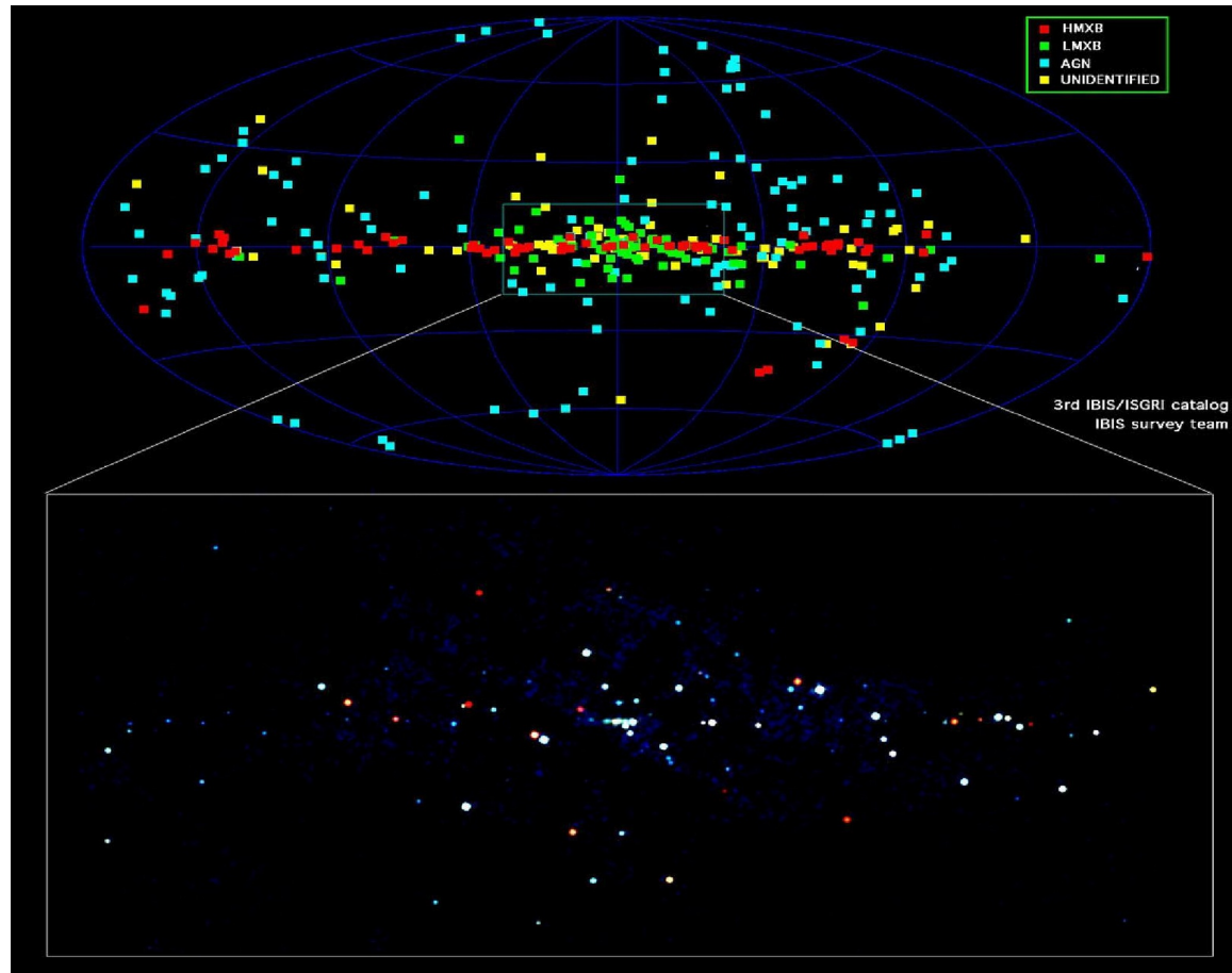
Figure 39: Densest objects seen by INTEGRAL. The red and green boxes represent dense objects discovered by INTEGRAL in our galaxy. The blue spots are supermassive black holes in the distant universe. The yellow spots are
