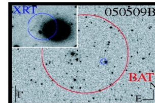
short GRBs
