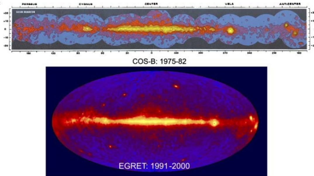
Fig. 5 Imaging with pair telescopes > 100 MeV. In the COS-B map, the Cygnus Region, Inner Galaxy, Vela Pulsar and Crab and Geminga Sources beyond the “galactic hole” between 210^\circ and 250^\circ galactic longitude are visible. In the EGRET map, extragalactic sources are added, like 3C279, PKS 0524 + 134, the LMC, PKS 0208-512, or 3C454.3
