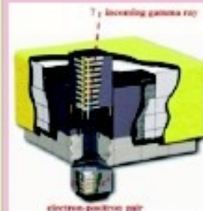
pair converters
