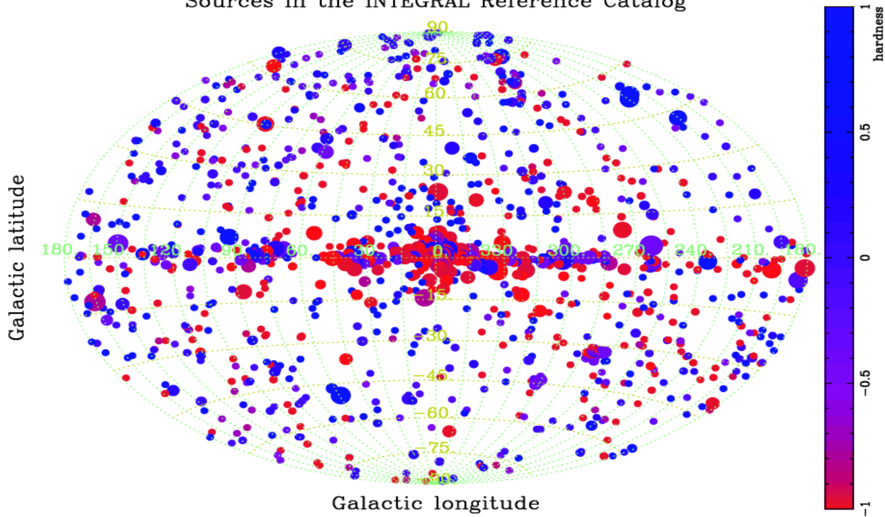
Sources in the INTEGRAL Reference Catalog
