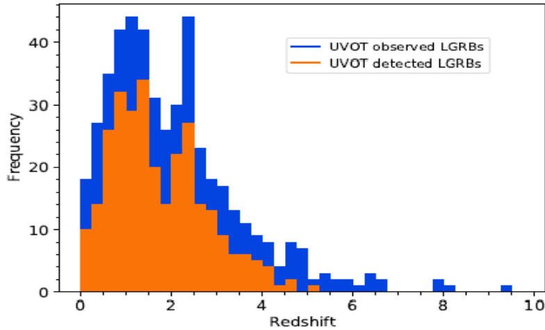
Figure 1. The redshift distribution of Swift /UVOT GRBs. The redshift distribution of long GRBs observed by Swift /UVOT is given in blue, while the redshift distribution of long GRBs detected by Swift /UVOT is given in orange.
