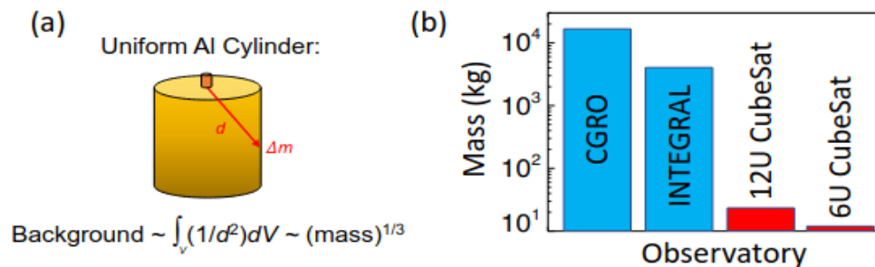
Fig. 1 (a) Instrumental background scales approximately as (\text{mass})^{1/3} . (b) CubeSat missions have 2-3 orders of magnitude lower mass than previous missions designed for MeV gamma-ray astronomy.
