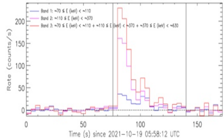
Fig. 2 GRB211019A lightcurve obtained by GRBAlpha [83]
