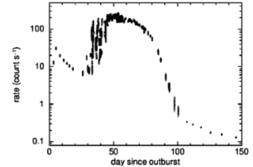
Figure 1: Left: ROSAT light-curve (0.1–2.4 keV) of V1974 Cyg (taken from Krautter et al., 1996 ), demonstrating the most detailed X-ray light-curve of a nova obtained before Swift. Right: The X-ray light-curve (0.3–10 keV) of RS Oph ( Osborne et al., 2005 ) from the first detailed Swift monitoring campaign of a nova. Only the first outburst are shown.
