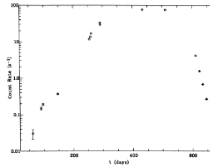
Figure 1: Left: ROSAT light-curve (0.1–2.4 keV) of V1974 Cyg (taken from Krautter et al., 1996 ), demonstrating the most detailed X-ray light-curve of a nova obtained before Swift. Right: The X-ray light-curve (0.3–10 keV) of RS Oph ( Osborne et al., 2005 ) from the first detailed Swift monitoring campaign of a nova. Only the first outburst are shown.
