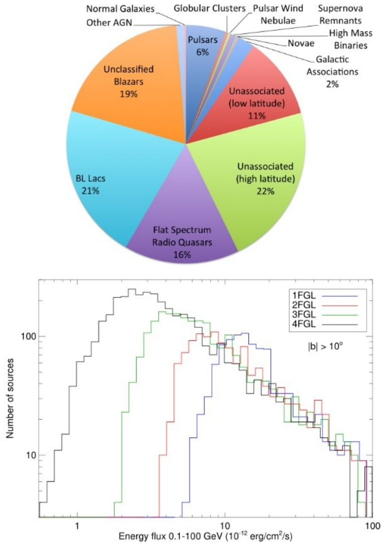
Figure 3. Distributions of the energy flux for the high-latitude sources ( |b| > 10^\circ ) in the 1FGL (1043 sources, blue), 2FGL (1319 sources, red), 3FGL (2193 sources, green) and 4FGL (3663 sources, black) catalogs, illustrating the approximate detection threshold.
