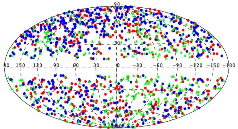
3 The sky distribution of the blazars listed in the 3LAC (Hammer-Aitoff projection), shown in Galactic coordinates (Ackermann et al. 2015a). Red circles FSRQs, blue circles BL Lacs, green triangles BCU candidates of uncertain type (BCUs)
